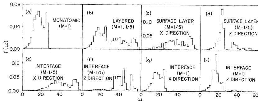
FIG. 2. Frequency distribution function f(\omega) and effective distribution functions f_\alpha(\omega; I_3) for (a) a monatomic slab-shaped crystal and (b)–(h) a layered structure. In this figure, M represents the masses of the particles; in the monatomic crystal, all particles have a mass of 1, and in the layered structure there are particles of mass 1 and mass \frac{1}{5} .
